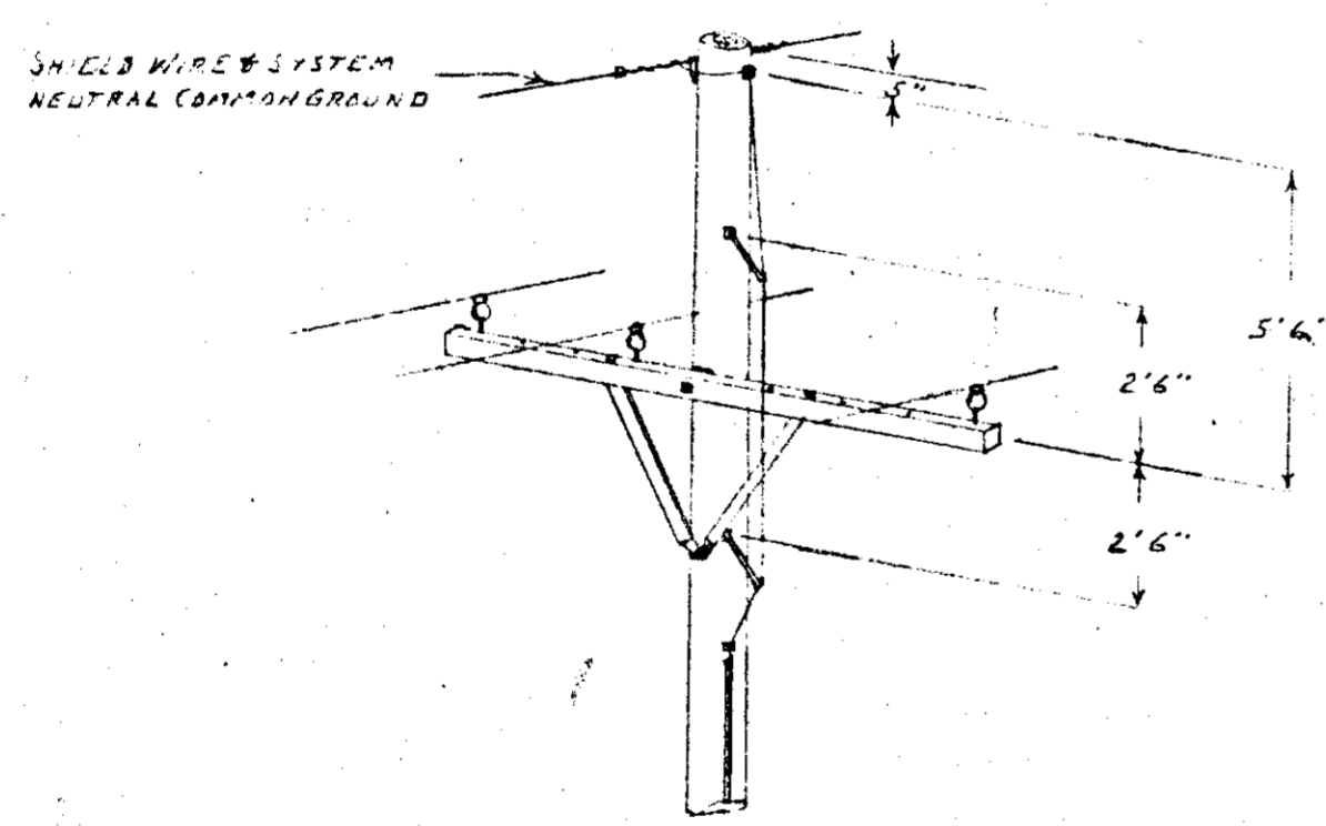
TYPICAL POLE TOP
